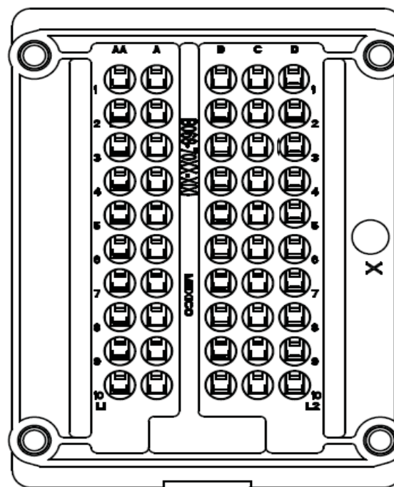
BOTTOM VIEW
