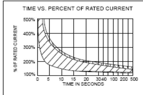
10 AMPS & BELOW TYPICAL CURVE 15 AMPS & ABOVE TYPICAL CURVE
