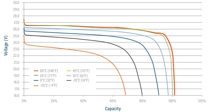
DISCHARGE VOLTAGE CHARACTERISTICS AT VARIOUS TEMPERATURES DISCHARGE 1C
