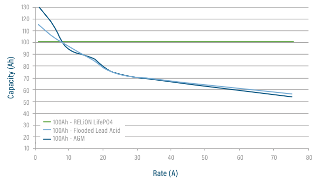
CAPACITY OF RELIION LiFePO4 vs. LEAD ACID at VARIOUS RATES OF DISCHARGE
